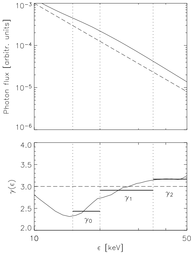
Fig. 1. Photon spectrum I(\epsilon) (upper panel) and spectrum index \gamma(\epsilon) (lower panel) for a modelled primary photon spectrum I_p(\epsilon) \sim \epsilon^{-3} for an isotropic source located at \mu = 0.8 . Primary I_p(\epsilon) and \gamma_p(\epsilon) are plotted with a dashed line and the observed I_o(\epsilon) and \gamma_o(\epsilon) with a solid line. Horizontal lines indicate spectral indices \gamma_0 , \gamma_1 , and \gamma_2 obtained by single power-law fits in the 15 - 20, 20 - 35, and 35 - 50 keV energy ranges, respectively.
